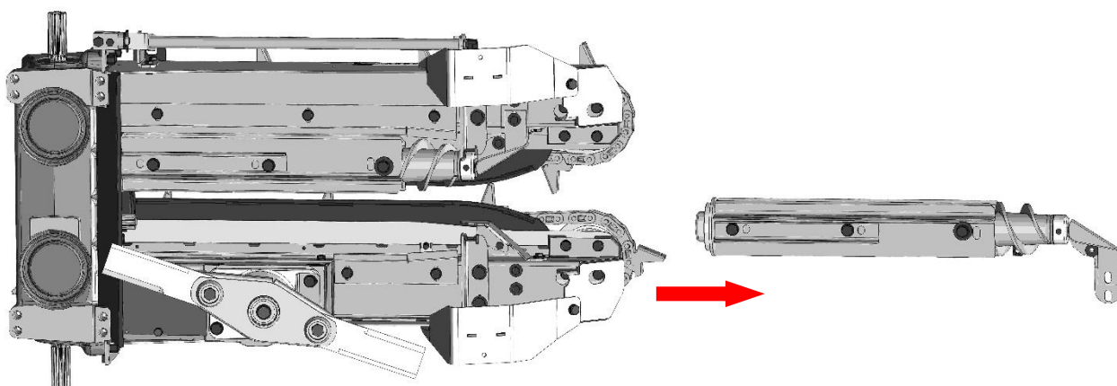
Fig.6 Dismantle the knife guard, remove the screws of the stalk roller holder.
