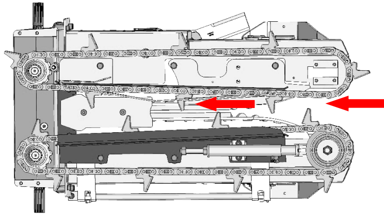
Fig.3 Push in the counter blade from the front as far as it will go.
