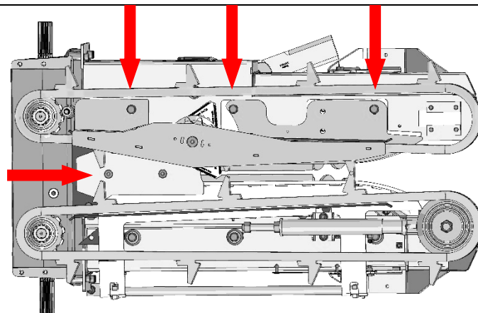
Fig.3 Push in the counter blade from the front as far as it will go.
