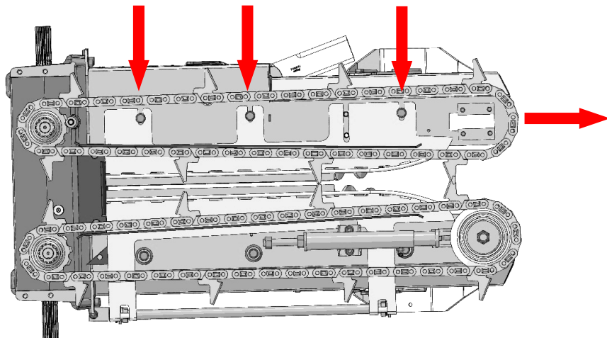
Fig.1 Push in the counter blade from the front as far as it will go.
