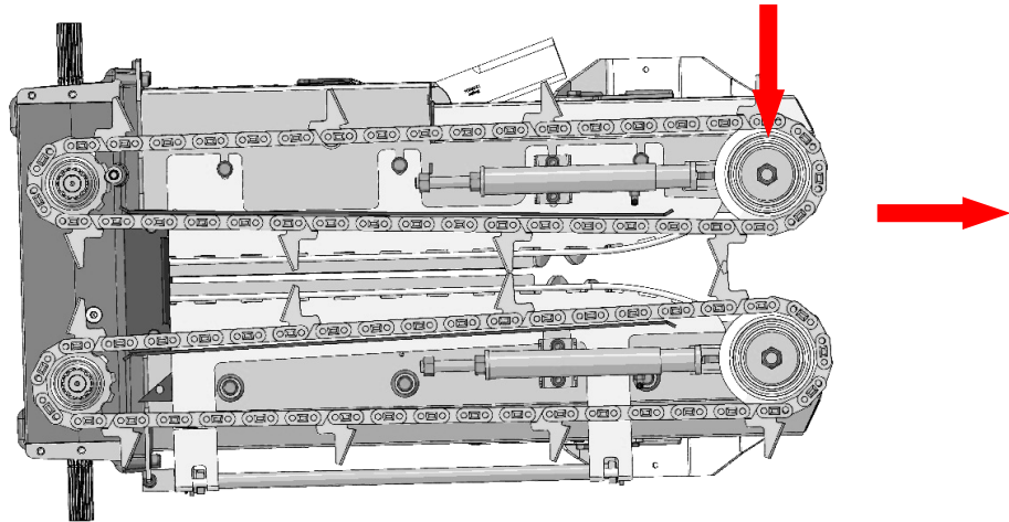
Fig.1 Push in the counter blade from the front as far as it will go.
