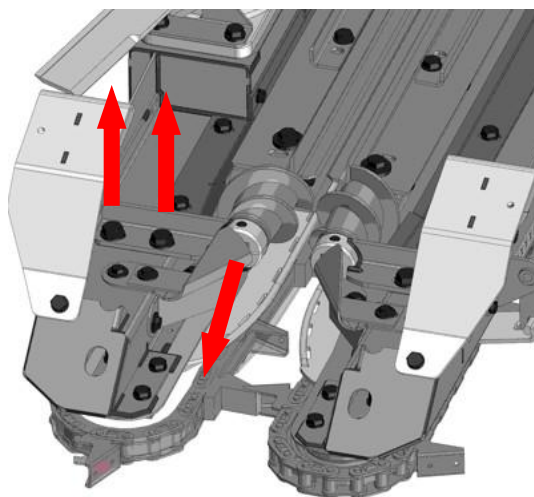
Fig.6 Dismantle the knife guard, remove the screws of the stalk roller holder.
